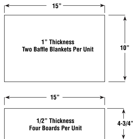
Figure 3 - Baffle Insulation Parts
