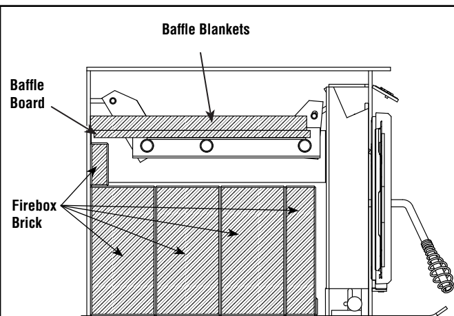
Figure 4 - Side Cut-A-Way View of Firebox
