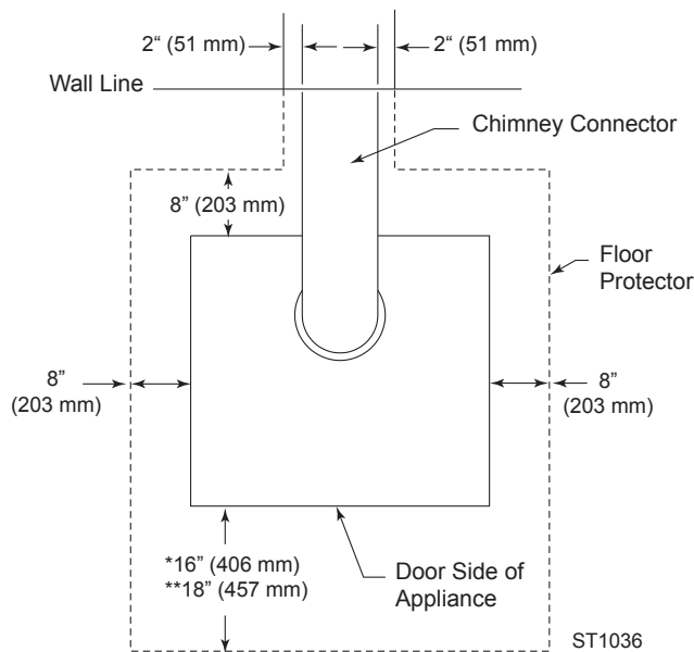
Figure 4 Floor Protector
