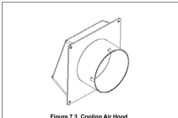
Figure 7.3 Cooling Air Hood
