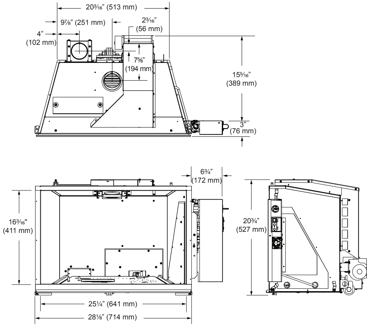
Figure 2 - VLI31 Fireplace Insert Dimensions
