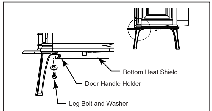
Figure 3.4 - Handle holder and heat shield positions.
