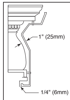
Figure 2.15 - A custom-formed mantel shield.
