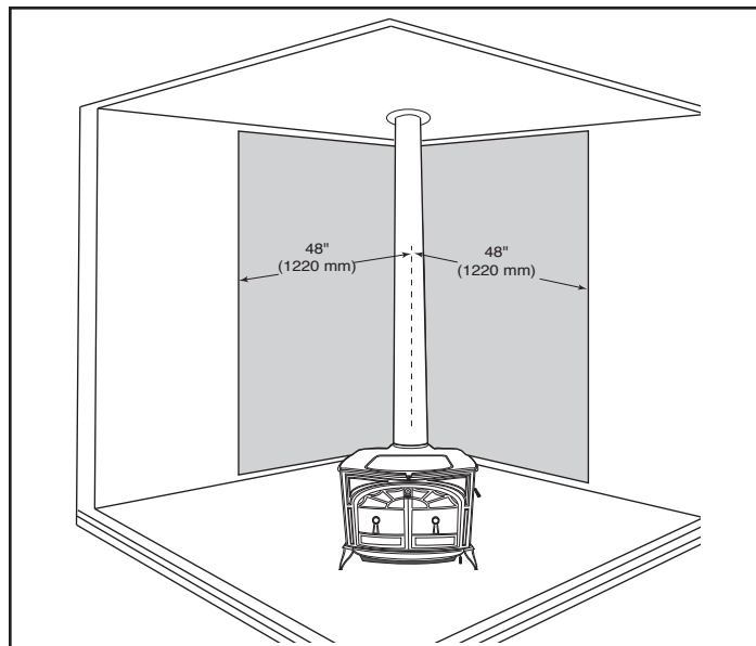
Figure 2.14 - Corner installation, vertical chimney connector, two wall shields. Reduced side clearances. Wall shield MUST meet at corner.
