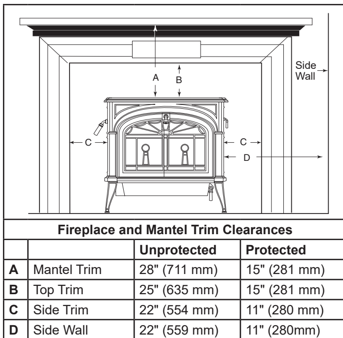
Figure 2.16 - Maintain clearances to combustible components of the mantel piece.
