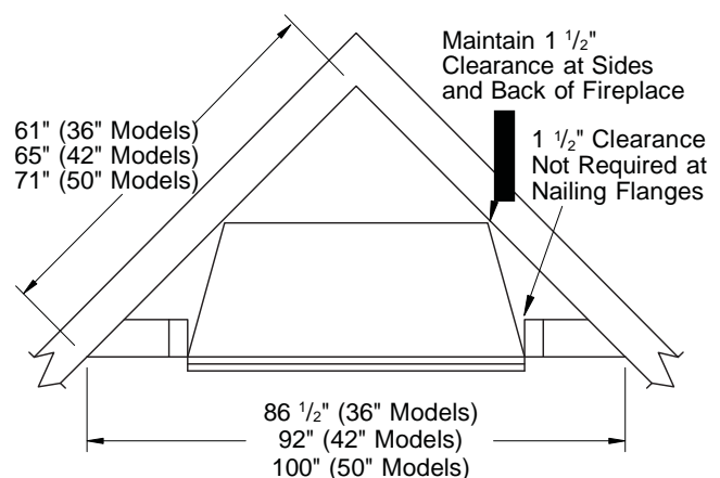
Figure 9 - Corner Installation
