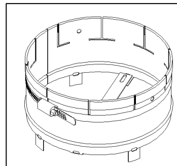
Figure 13: Liner Adaptor
