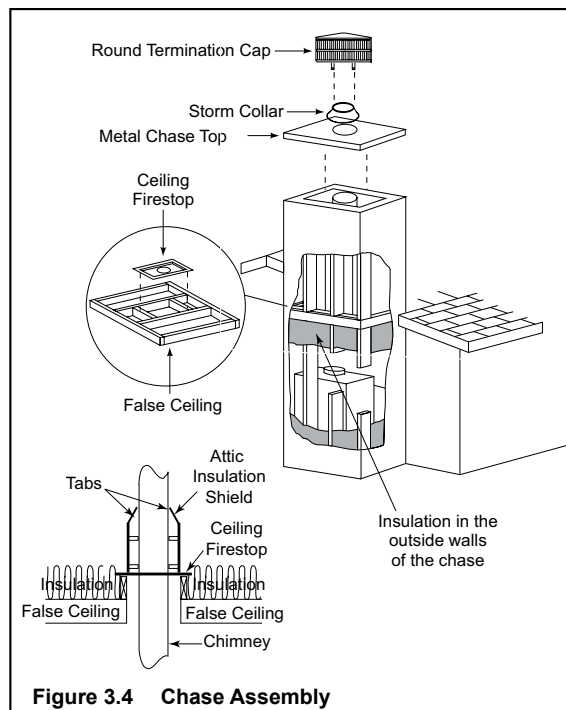
Figure 3.4 Chase Assembly
