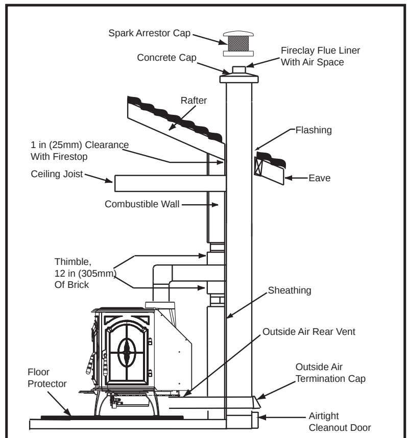
Figure 8.1 Masonry Chimney
