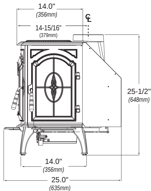
Side View With Fuel Door
