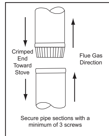
Figure 19.2 Chimney Connector (Stove Pipe)
