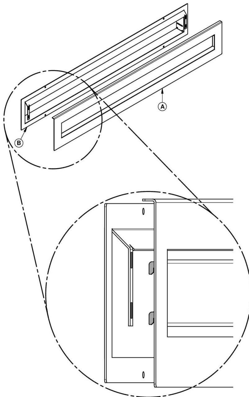
Figure 14 : Installation of the louvered face
