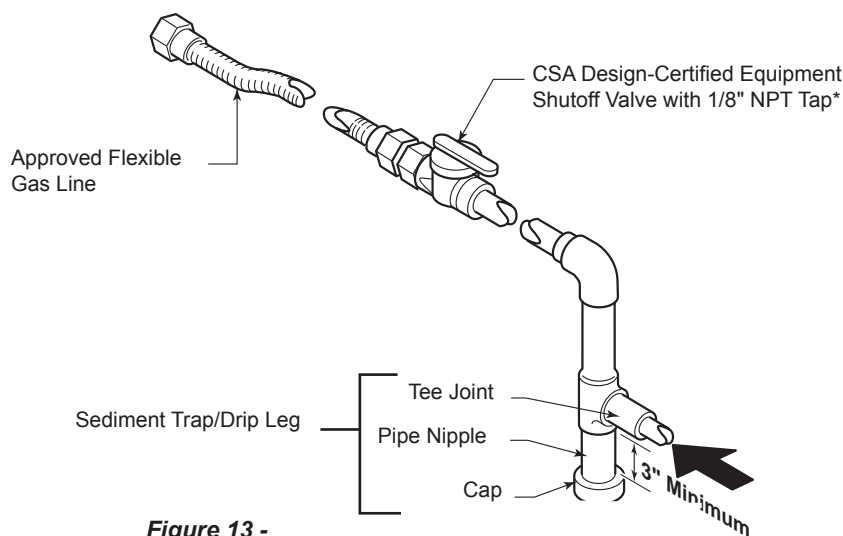
Figure 13 - Gas Connection
