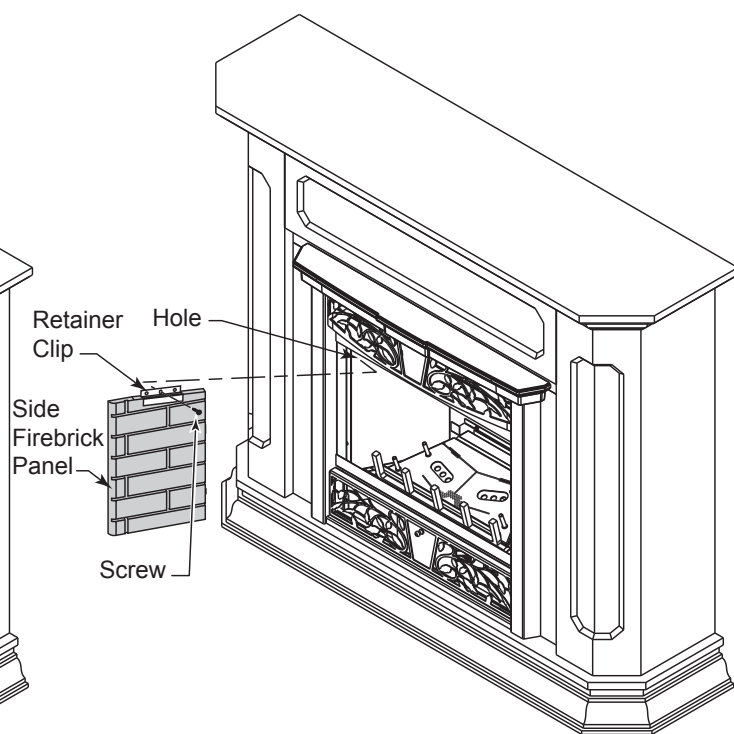
Figure 11 - Install Side Firebrick Panel
