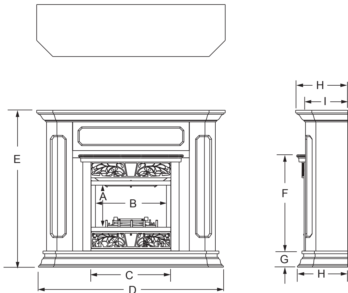
Figure 2 - Firebox Dimensions
