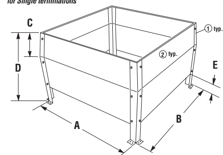
CTS0-33/44 Shrouds for single terminations
