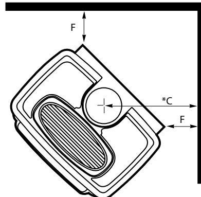
Top View / Corner Clearances
