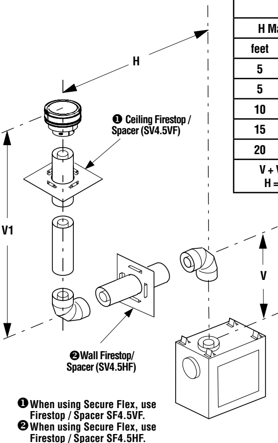
Figure 31 - Top Vent - TWO 90 DEGREE ELBOWS
