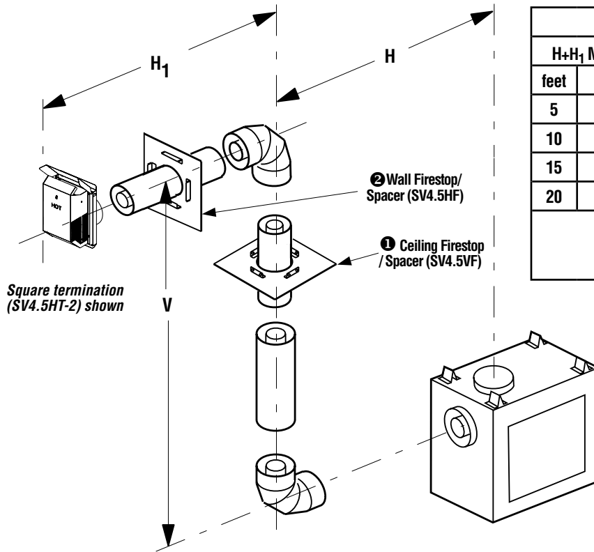
Figure 45 - Side Vent, TWO 90 DEGREE ELBOWS
