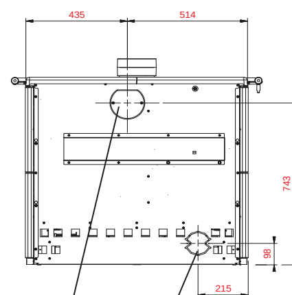
ROSA XXL UL-C Steel - 202 kg
