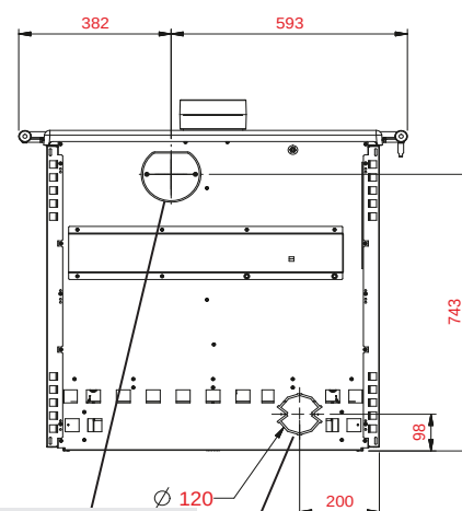
ROSA XXL UL-C Stone - 275 kg
