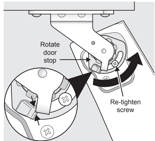
Re-tighten screw
