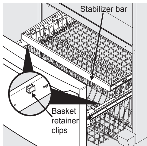
Two freezer baskets Figure 44
