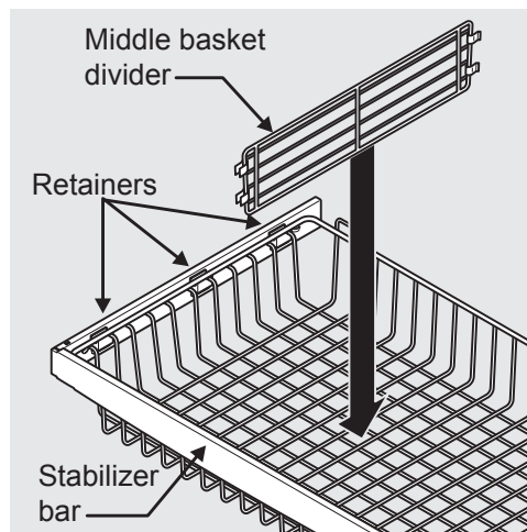
Upper basket divider Figure 46
