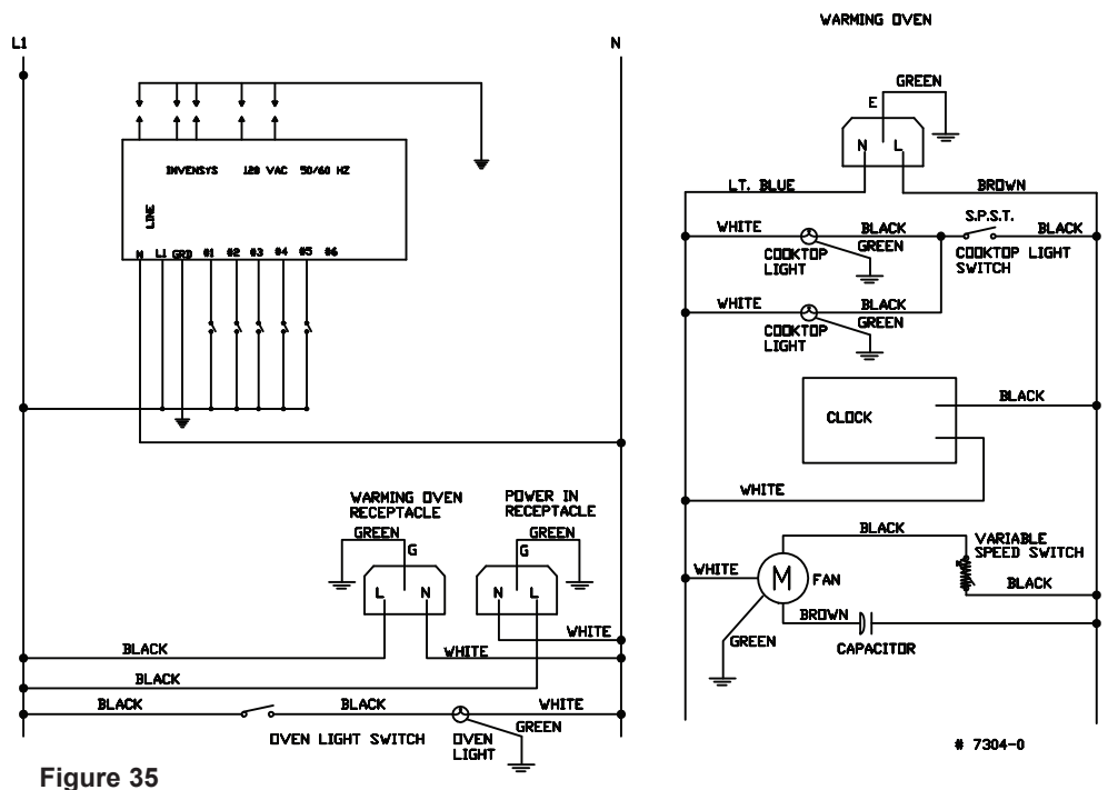
9200 WIRING DIAGRAM-N.A.
