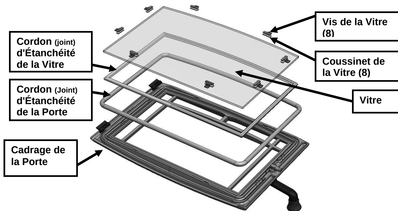
Figure 15: Porte Frontale
