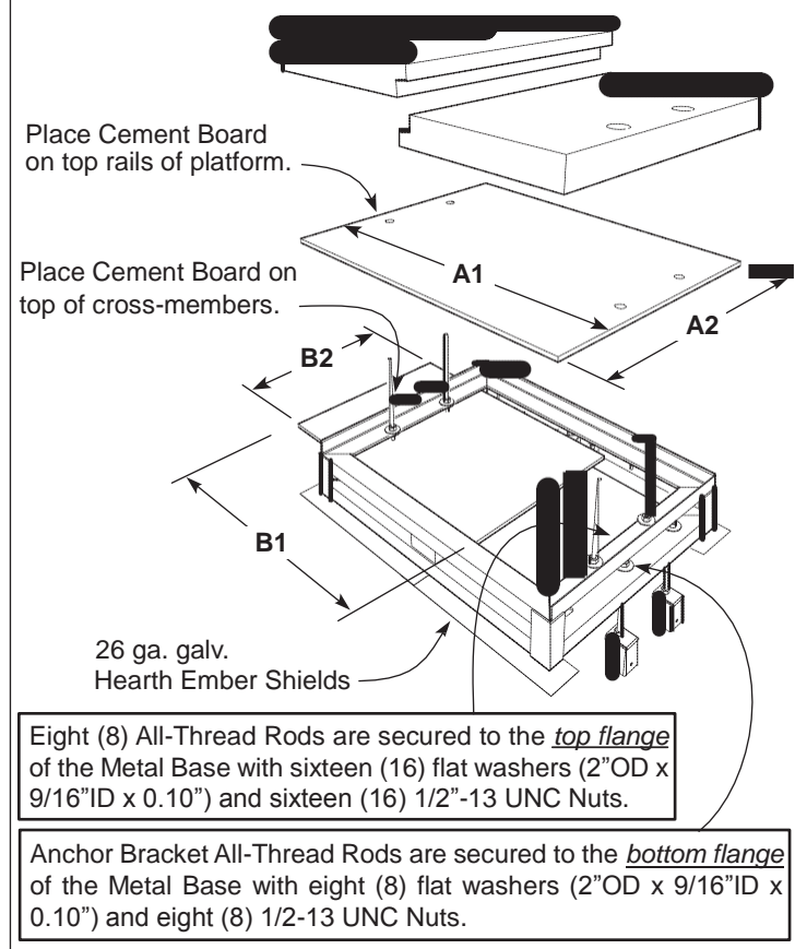
Figure 17 Metal Base Assembly
