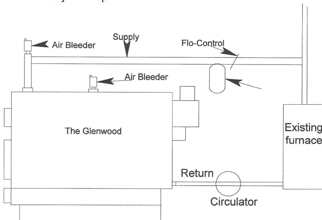
Primary Hookup
