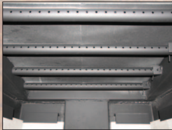
Secondary Air Tubes in Firebox save you money by burning the smoke produced, giving longer life to your fire.
