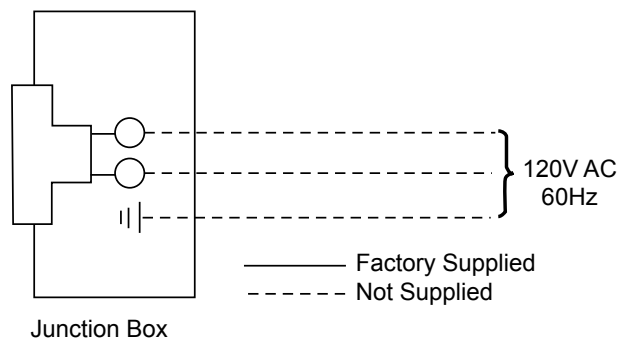
Junction Box Wiring Diagram
