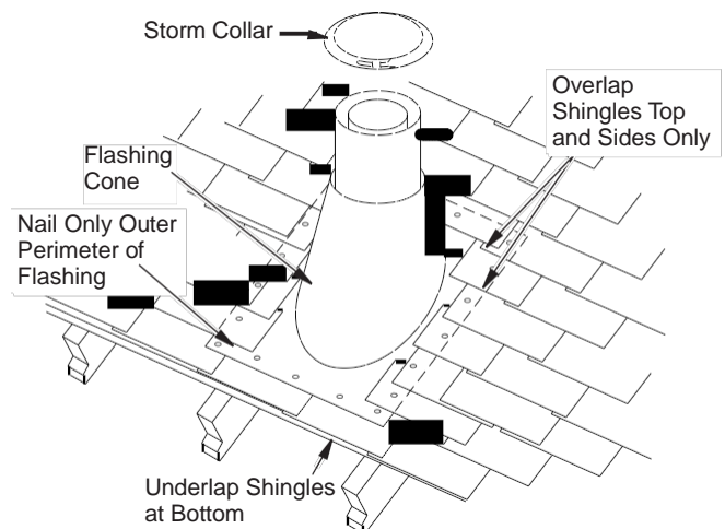
Figure 13 - Flashing Installation
