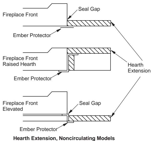
Figure 3 - Hearth Extension
