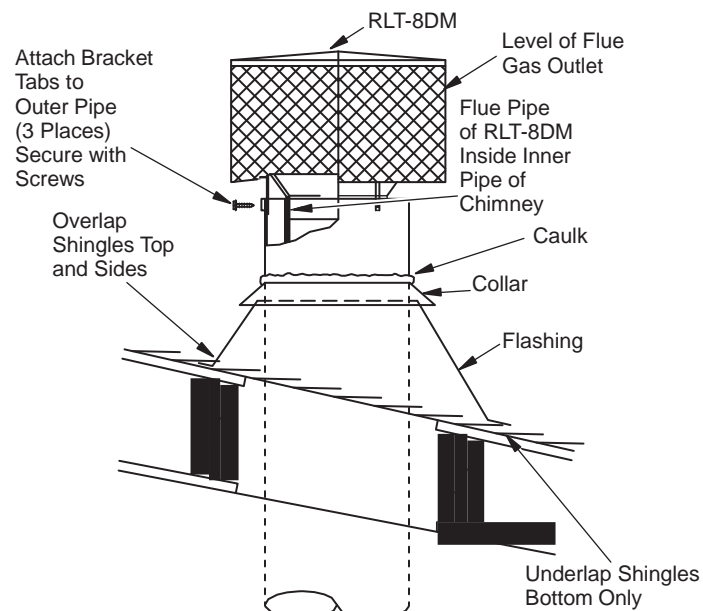
Figure 15 - Termination
