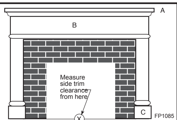
Fireplace Clearances
