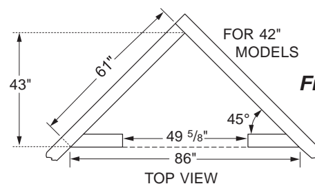
Figure 7 - Rough Opening for Installing in Wall
