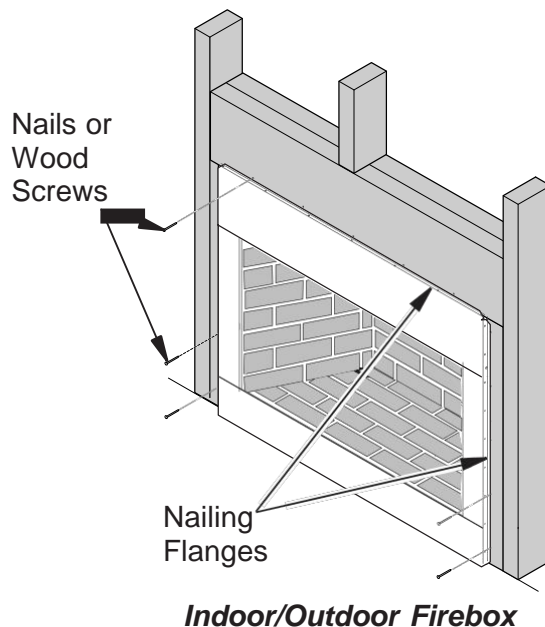
Figure 8 - Attaching Firebox to Wall Studs
