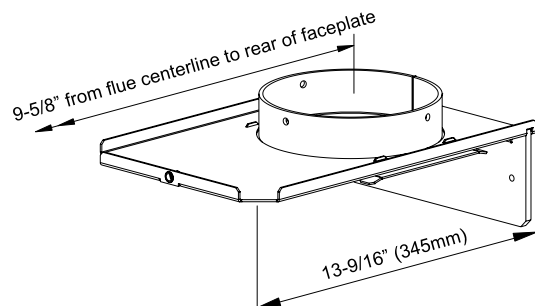
6" (152mm) Diameter STANDARD FLUE ADAPTOR (171-932)
