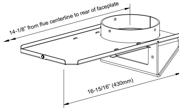
6" (152mm) Diameter OFFSET FLUE ADAPTOR (171-936)
