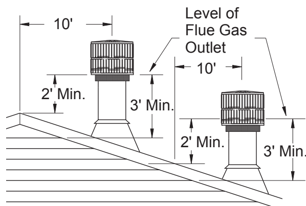
Figure 20 - 10 Foot Rule
