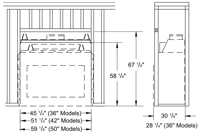
Figure 4 - Framing Dimensions
