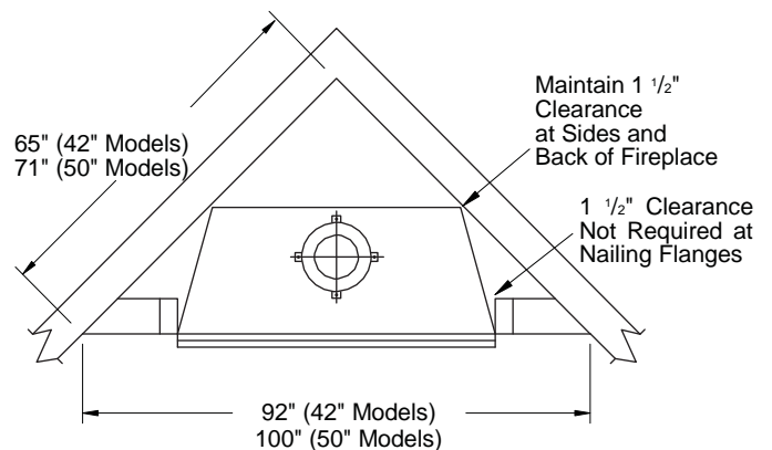
Figure 4 - Corner Installation
