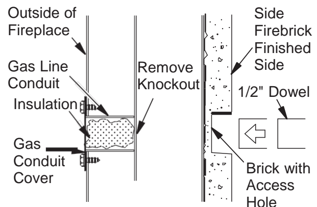
Figure 23 - Gas Line Access
