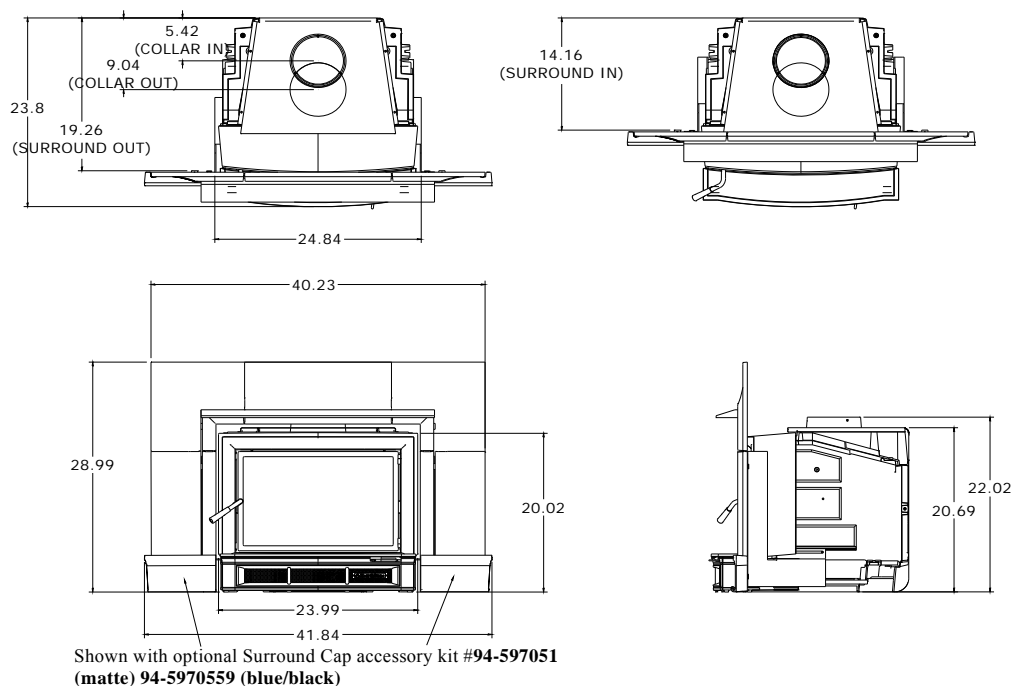
Figure 1 Morgan Dimensions
