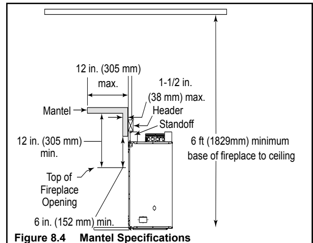
Figure 8.4 Mantel Specifications
