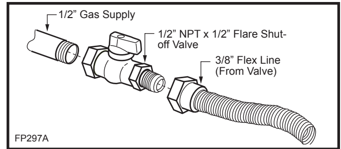
Fig. 7 Typical gas supply installation.
