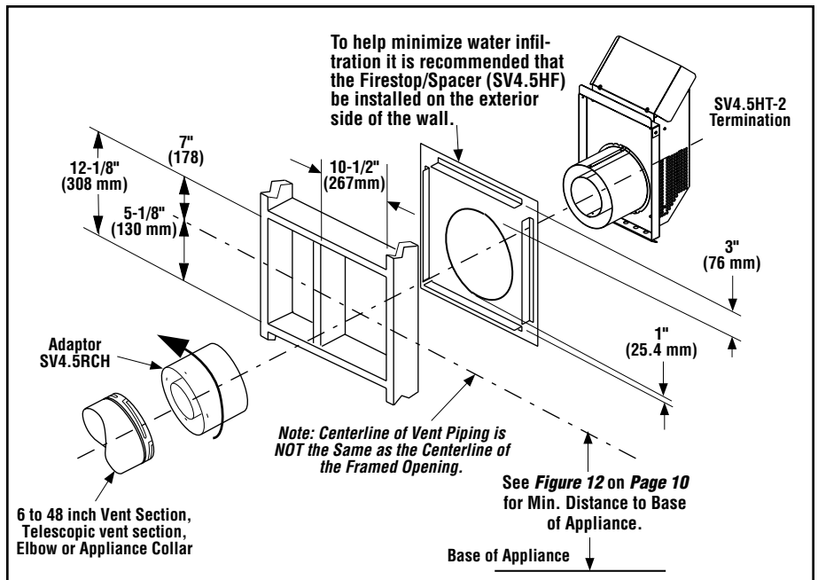
Figure 40: Installing the Square Horizontal Termination (SV4.5HT-2)
