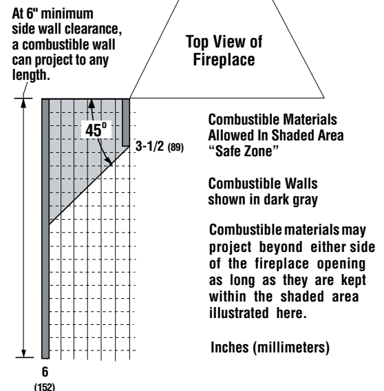
Figure 9: Minimum Distance to Side Wall
