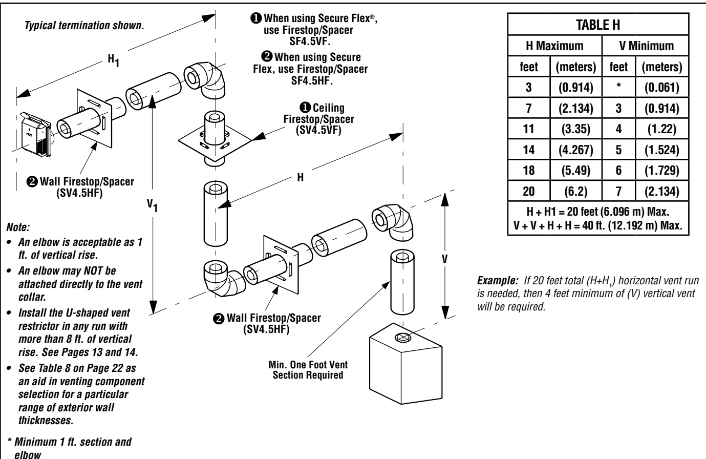
Figure 46: Top Vent - THREE 90-DEGREE ELBOWS
