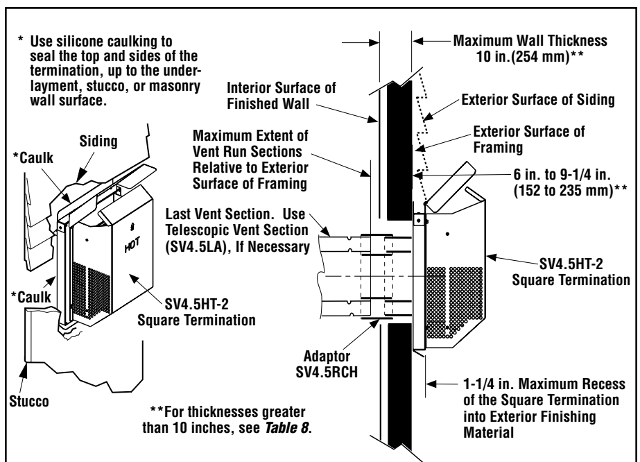
Figure 41 Venting Connection and Exterior Wall Recessing of the Horizontal Square Termination (SV4.5HT-2).
