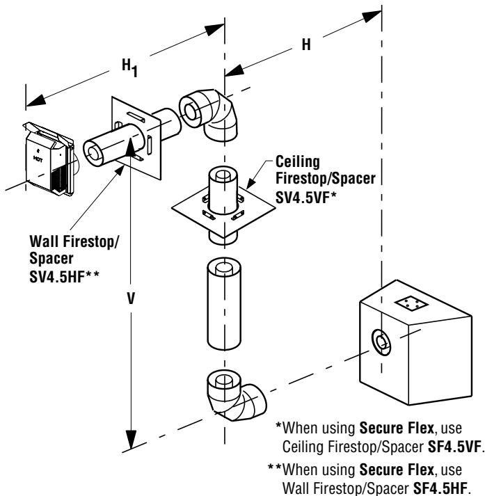
Figure 45: Rear Vent - TWO 90-DEGREE ELBOWS
