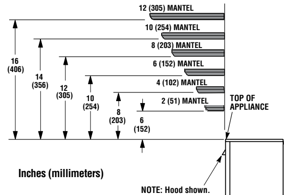
Figure 8: Minimum Mantel Clearances
