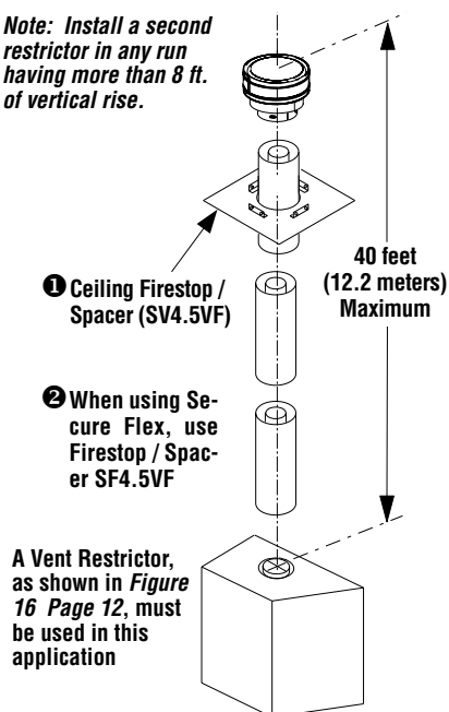
Figure 25 - Top Vent - STRAIGHT
