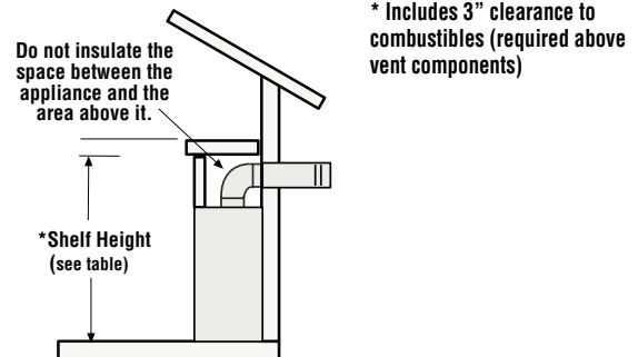
Figure 8 - Shelf Height Minimum Clearances With Top Venting
