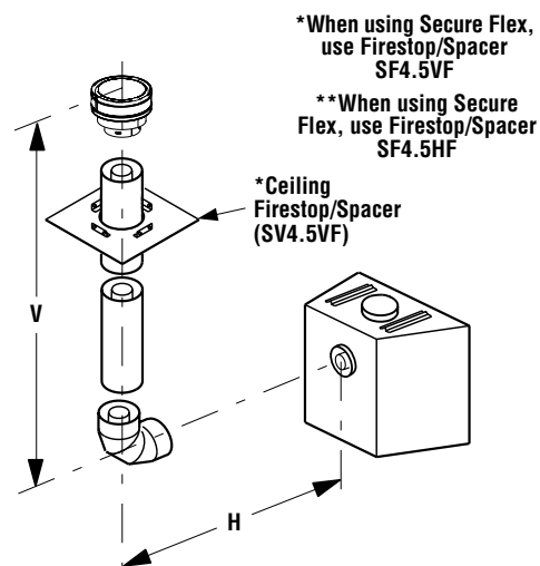
Figure 30 - Rear Vent - ONE 90 DEGREE ELBOW
