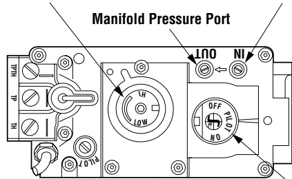
SIT Millivolt Gas Valve
