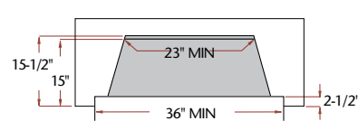
Minimum Fireplace Dimensions
