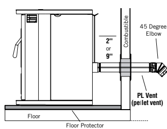
Parallel Through the Wall View
