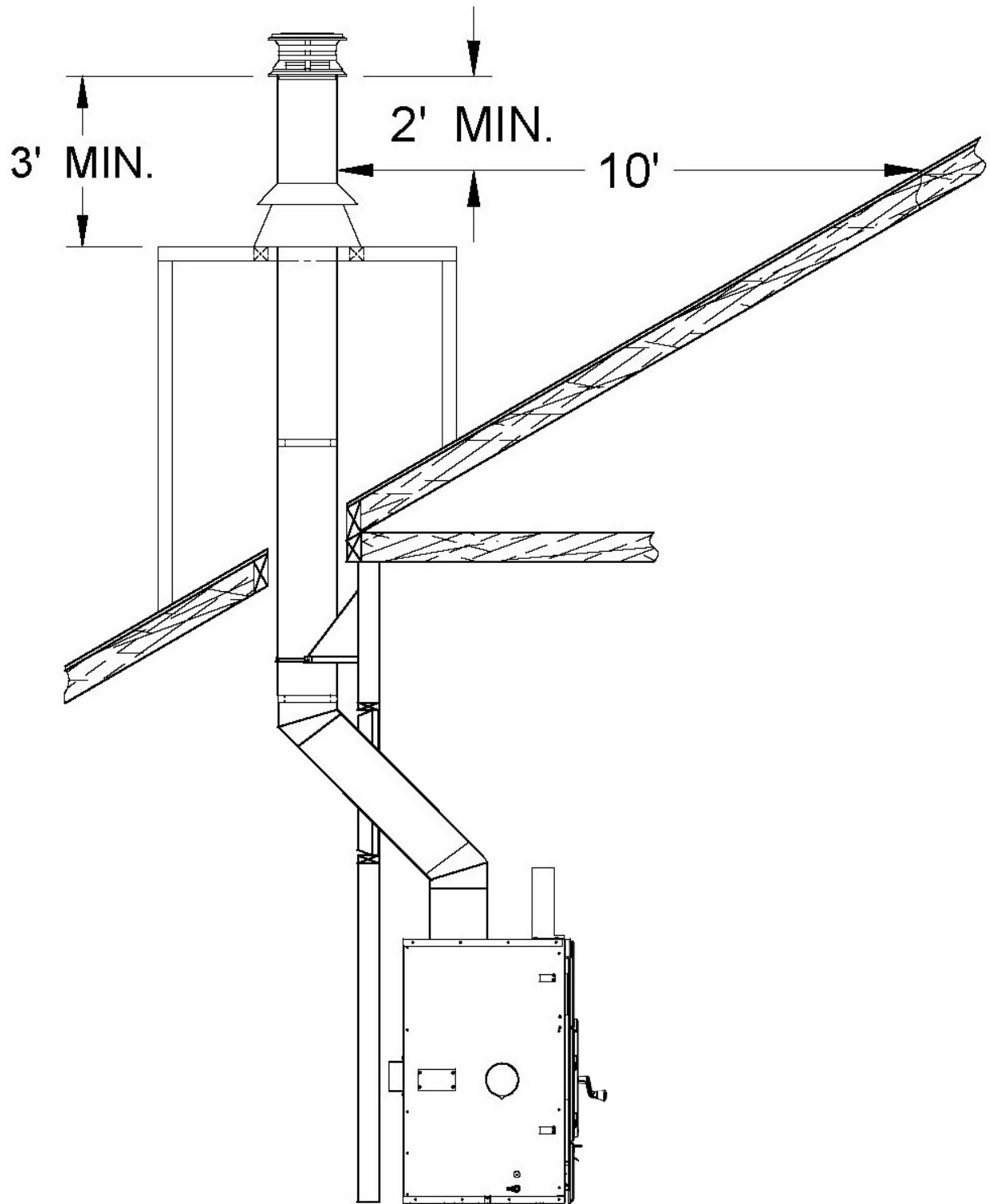
Figure 45 – Example of a combustible chase enclosure installation above the roof
