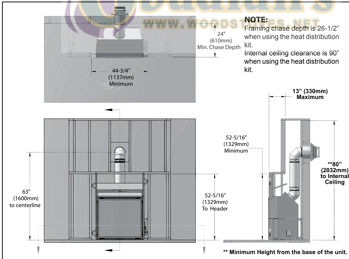
Typical Framing for Internal Chase - General
