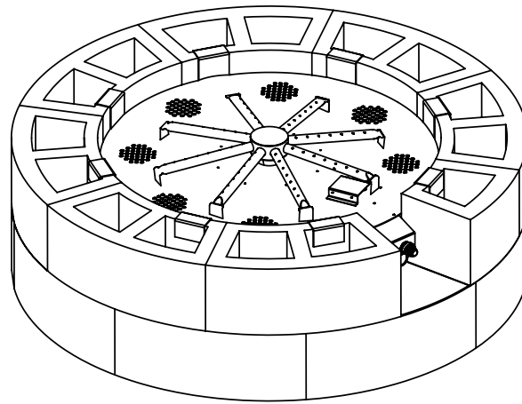
Star burner
