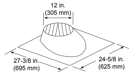
RF370 - Roof Flashing Flat to 6/12 Pitch
