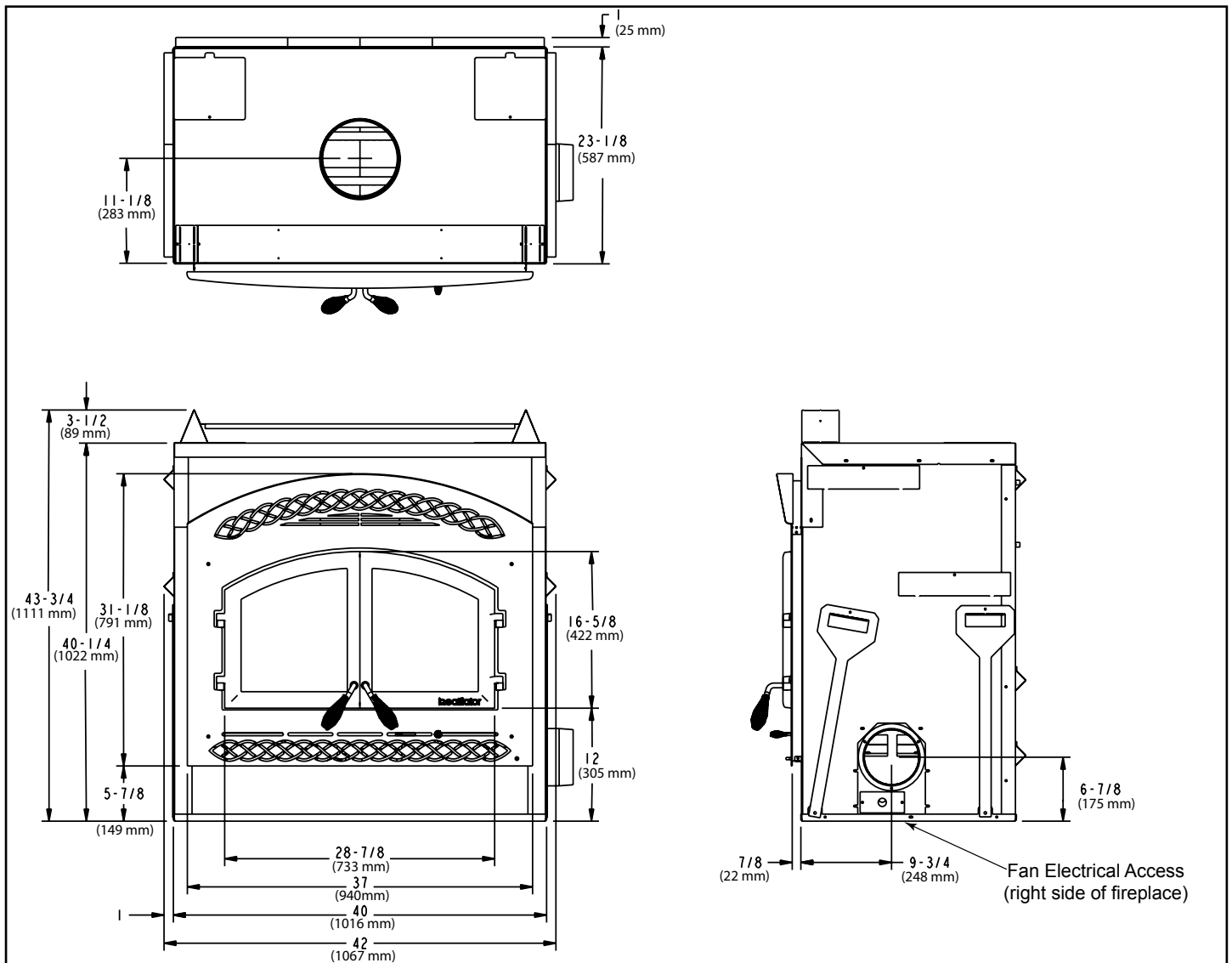
Figure 3.1 Fireplace Dimensions
