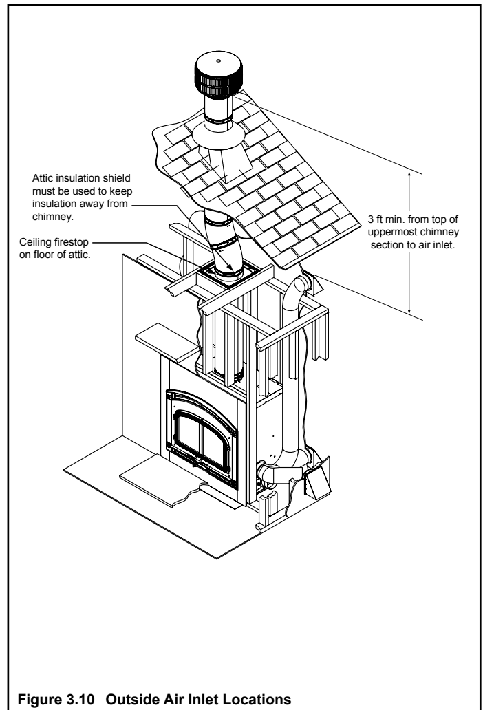
Figure 3.10 Outside Air Inlet Locations
