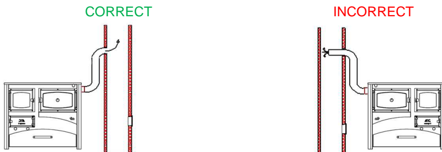
(Fig. 6) Connecting the flue pipe (shuttle) to the chimney
